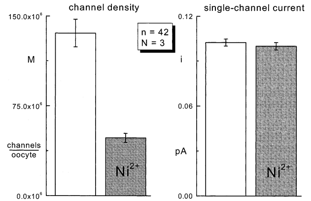
Fig. 5. Data from noise analysis. \text{Ni}^{2+} drastically reduced the number ( M ) of active channels by directly inactivating rENaCs (left panel), while single-channel current ( i ) was not affected. Shown are pooled data from 42 oocytes from three animals.
